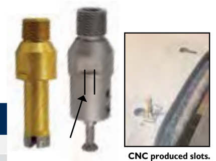
CNC produced slots.
