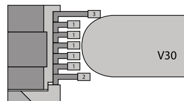
Spacer Blade Lock (Spacer not required on most configurations.)
