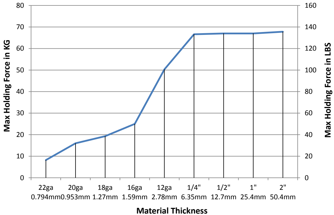
Magswitch MagSquare 165 Breakaway vs. Thickness
